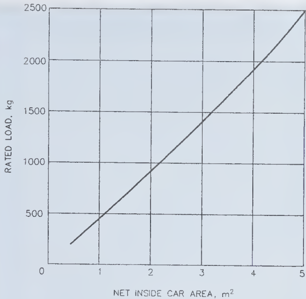
FIG. 7 MINIMUM RATED LOADS FOR PASSENGER LIFT CAR
