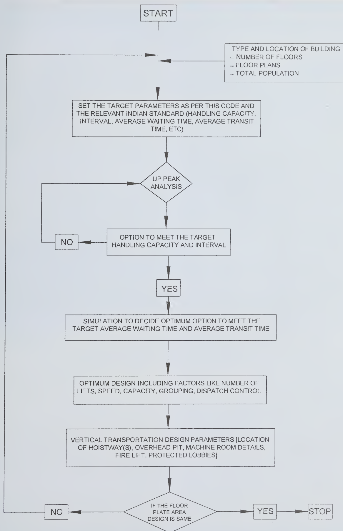
FIG. 1 TYPICAL FLOWCHART ON PRELIMINARY DESIGN OF LIFTS
