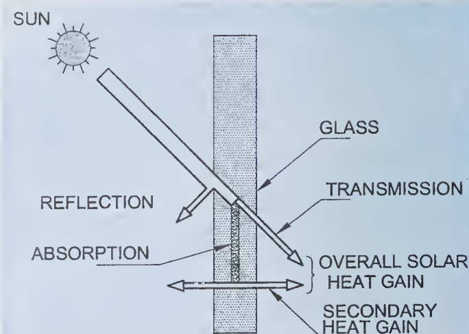
FIG. 2 MECHANISM OF SOLAR HEAT GAIN
