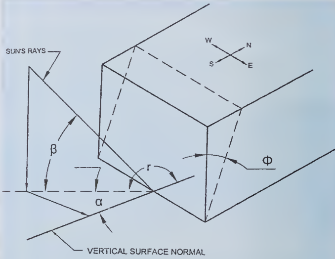
FIG. 12 DEFINITION OF SOLAR ANGLES
