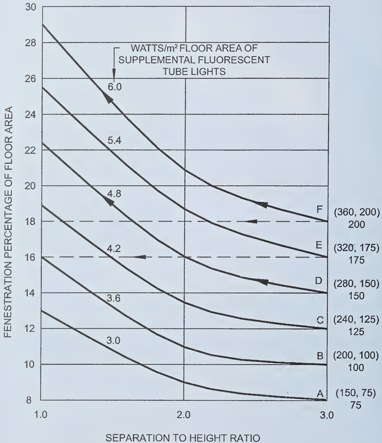
FIG. 4 NOMOGRAPH FOR DAYLIGHTING AND SUPPLEMENTAL LIGHTING DESIGN OF BUILDINGS
